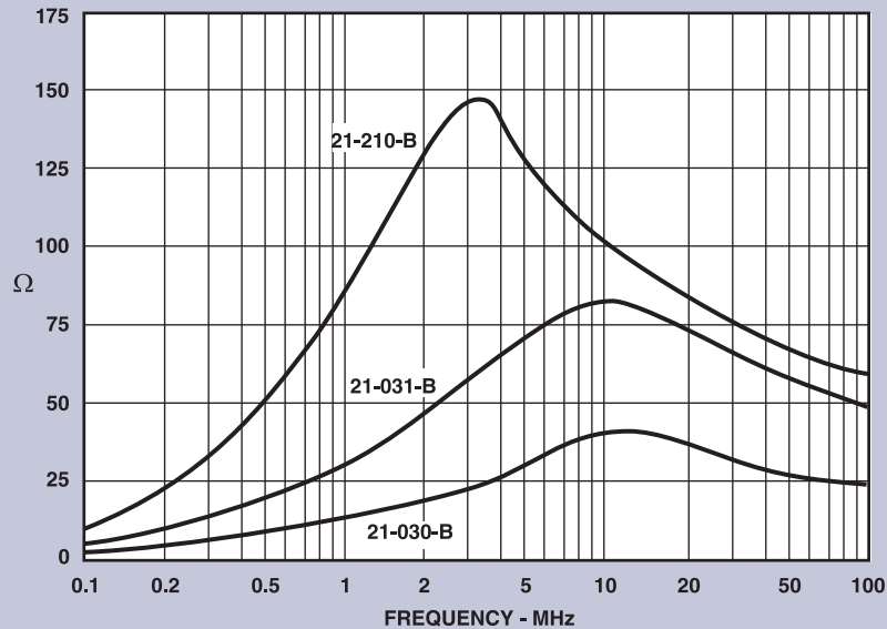
IMPEDANCE vs FREQUENCY FOR VARIOUS SIZES
